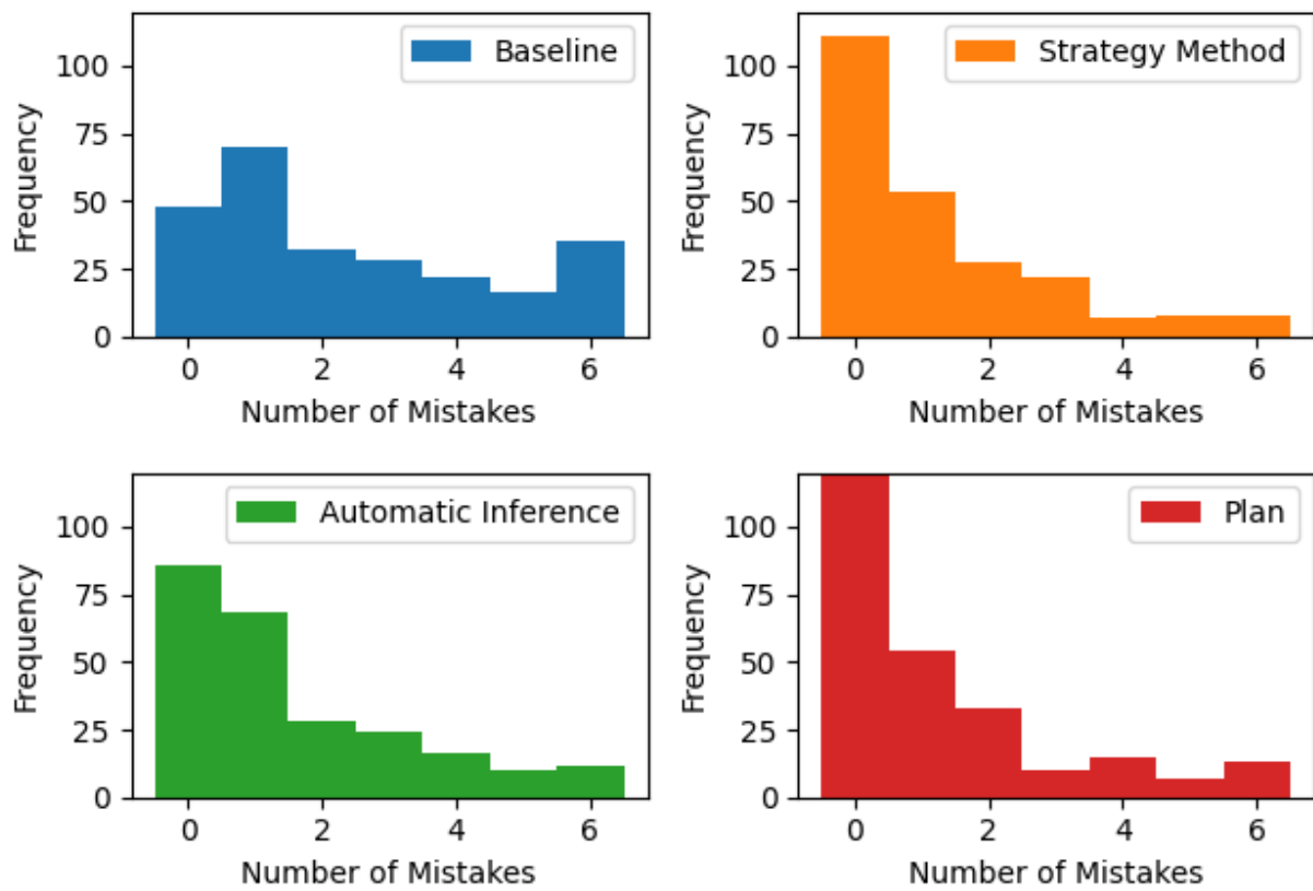
Figure A.6: The distribution of total screening mistakes participants make by treatment.
